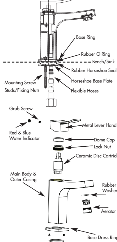
Linear Basin Mixer Illustrated
